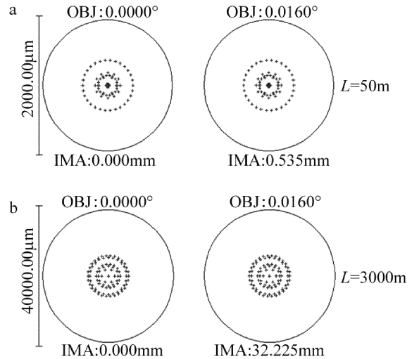
Fig. 3 Spot diagrams of the antenna in different distances at 20°C
