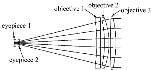
Fig. 2 Structure diagram of optical antenna
