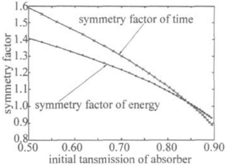
Fig 4 Relationship between the symmetry factor and T_0
