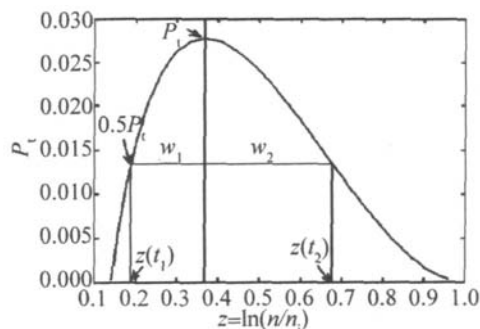
Fig 1 Temporal profile of a single pulse P_i versus the time-dependent variable z
