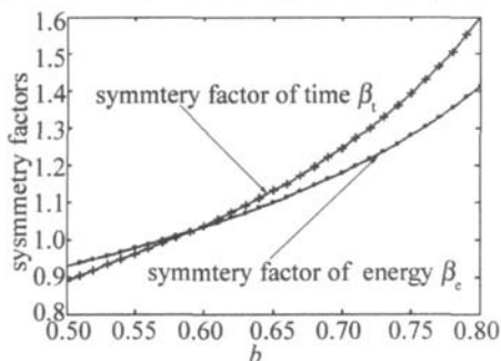
Fig. 7 Relationship between the symmetry factors and parameter b
