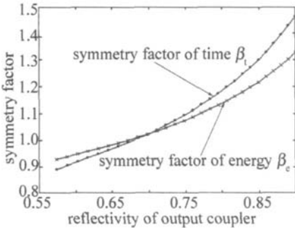
Fig 5 Relationship between the symmetry factor \beta and R
