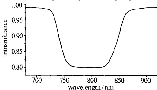
Fig 4 The profile of our grating
