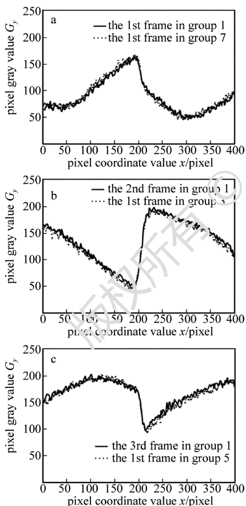
Fig. 7 Contrast of grayscale curves in the 200th column of each group a—the 200th column of the 1st frame in group 1 and the 1st frame in group 7 b—the 200th column of the 2nd frame in group 1 and the 1st frame in group 3 c—the 200th column of the 3rd frame in group 1 and the 1st frame in group 5
