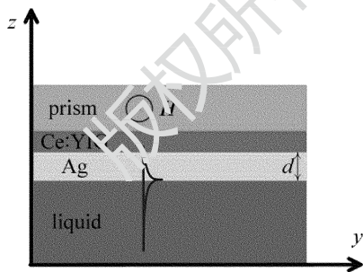
Fig. 1 Cross-section of magneto-optical structure in Cartesian coordinate system
