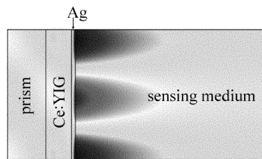
Fig. 2 Magnetic field distribution of MOSPR sensing system
