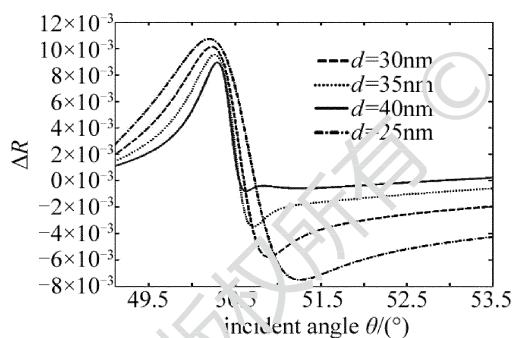
Fig. 4 Relationship between \Delta R and incident angle
