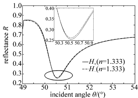
Fig. 3 Relationship between reflectance R and incident angle
