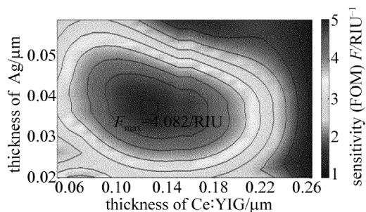
Fig. 5 Relationship between thickness Ag and thickness of Ce:YIG at 980nm
